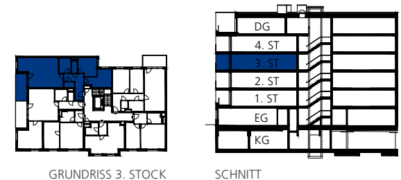
GRUNDRISS 3. STOCK
