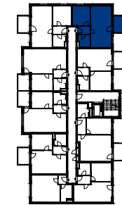
GRUNDRISS 3. STOCK
